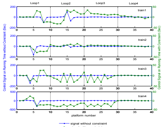
Figure 6. Control signal for MPC and constrained MPC.
