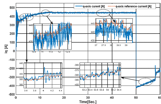
Figure 12. The reference and actual waveforms of the q-axis current i_{sq}
