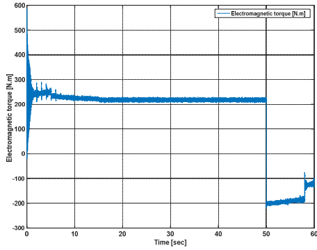
Figure 14. The electromagnetic torque produced by the PMSM
