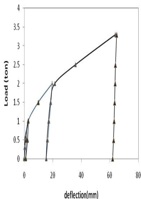
Figure 3. Plate load test for loose sand
