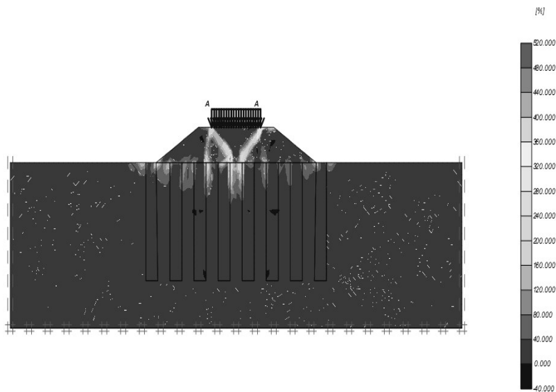
Figure 8. Failure surface of reinforced subgrade
