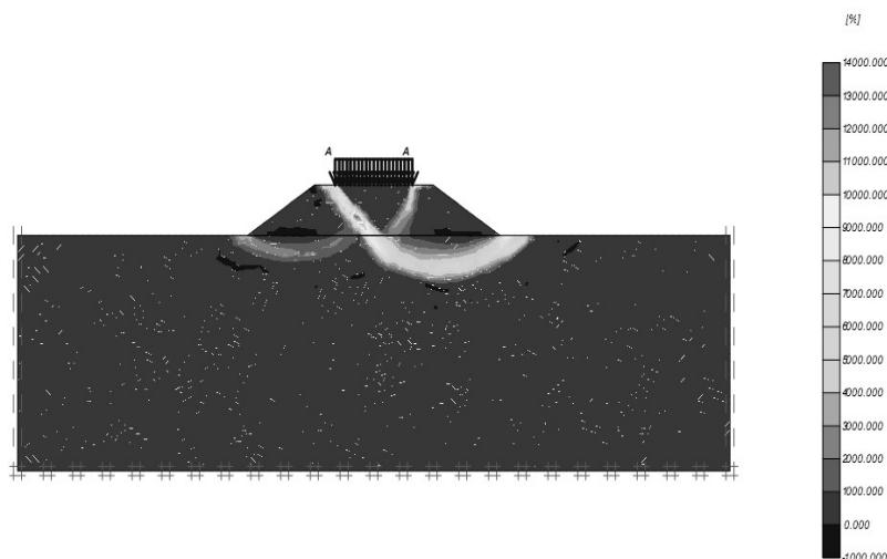
Figure7. Failure surface of unreinforced subgrade
