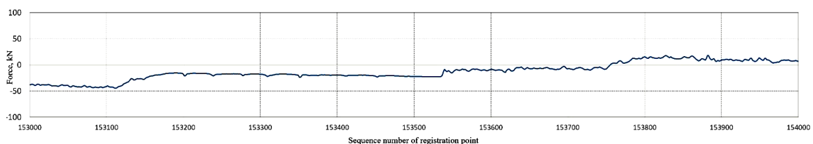
Figure 8. Longitudinal forces in urban electric train intercar linkage during acceleration
