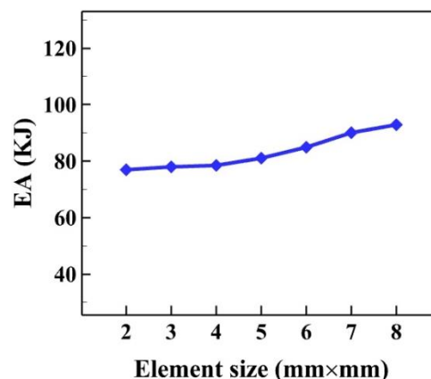
Figure 5. The mesh sensitivity analysis for the tube with trimmed diaphragms.
