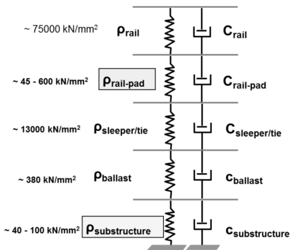
Figure 1. Cross section of a classic ballasted track (left) with the terminology according to the International Union of Railways [2] and schematic representation of the track as a combination of springs and dashpots (right)
