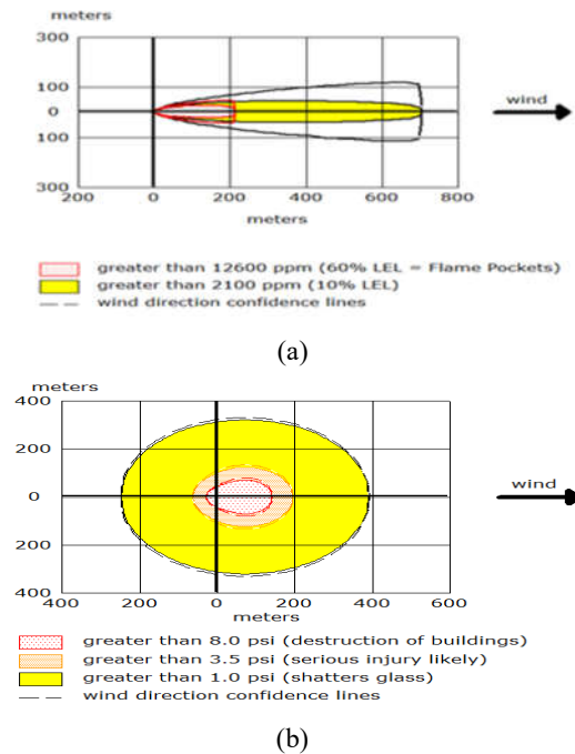
Figure 1. Definition of impact zones of propane, a: flammable zone, b: overpressure wave zone Figure 2(a)
