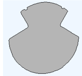
Figure 2. Contact wire cross-section
