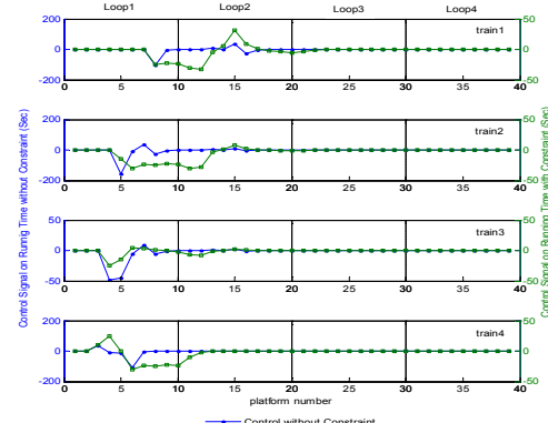
Figure 3. Control signals for LQR and constrained LQR
