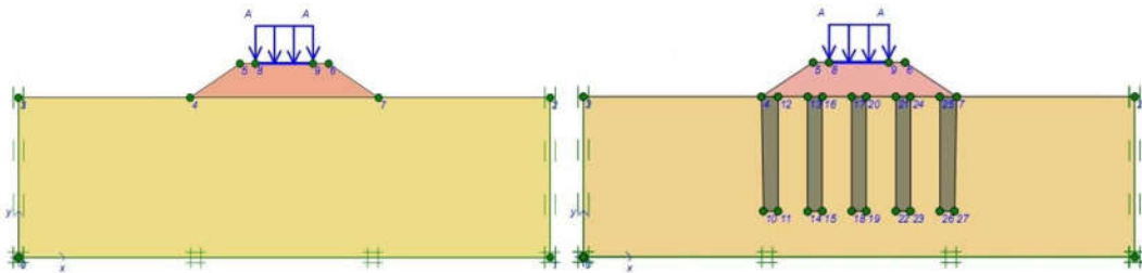
Figure 6. Embankment on a loose sandy soil in two situations of with and without columns
