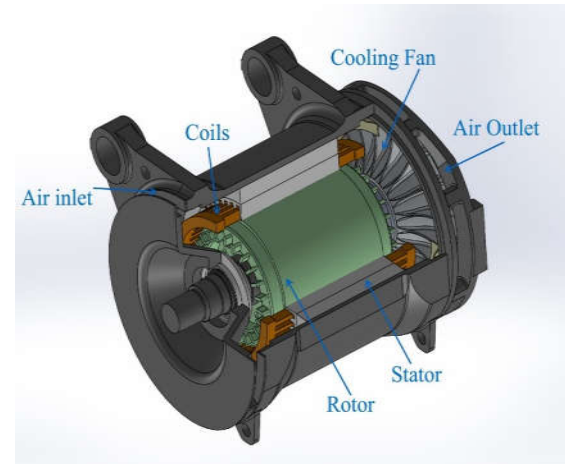
Figure 1. Computational Domain
