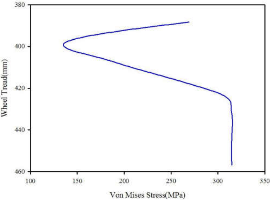
Figure 4. Von Mises stress according to wheel tread
