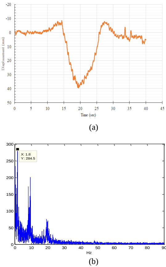
Figure 13. (a) Midspan displacement acquired through DIC (Train Passage Direction: Left to Right-Speed 65 Km/h), (b) FFT of the obtained midspan displacement data using DIC
