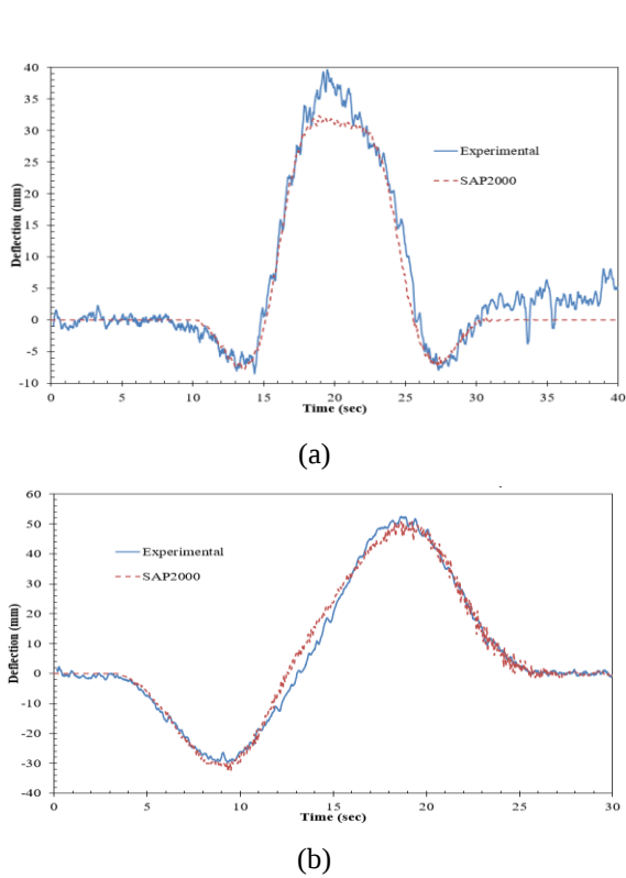
Figure 12. 3D Comparison of the displacements obtained from DIC and analytical model (a) Displacement of Mid span (Train Passage Direction: Left to Right-Speed 60 Km/h) (b) Displacement of Section 1(Train Passage Direction: Right to Left-Speed 55 Km/h)
