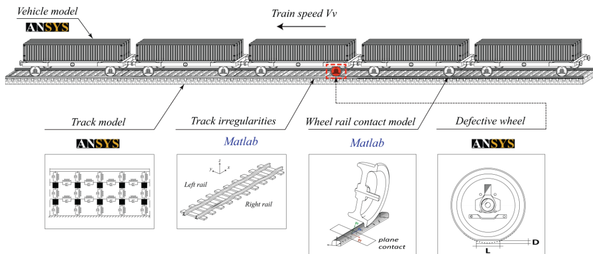
Figure 3. Train-track system
