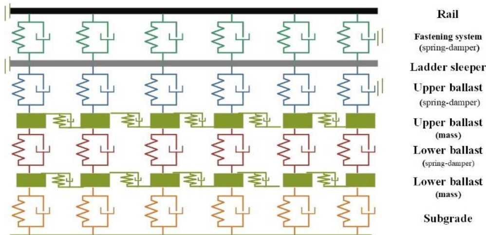
Figure 1. Schematic of the longitudinal model of the four-layer ladder track.
