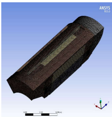
Figure 2. Generated Grid
