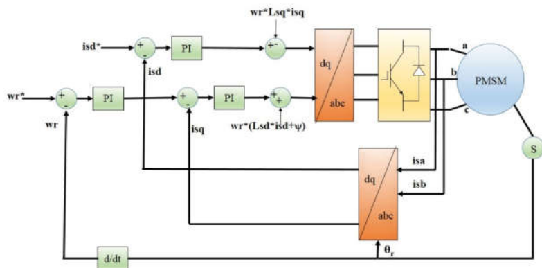
Figure 1. General block diagram of FOC strategy
