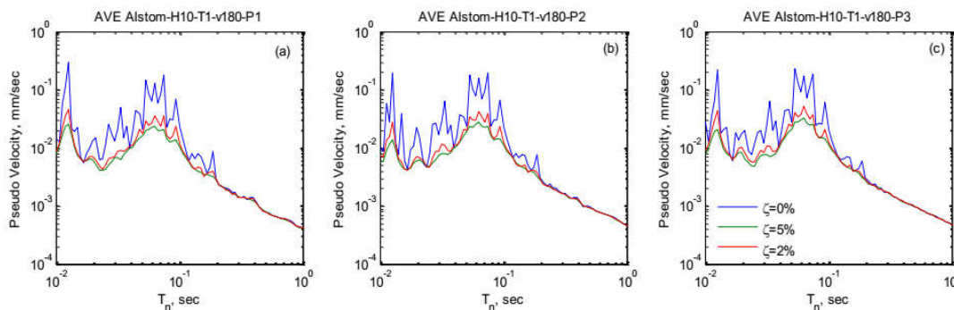
Figure 4. Pseudo-velocity spectra of a SDF system under passage of AVE Alstom train with velocity 180 km/h, tunnel depth 10 m and soil type I, (a) at the point P1, (b) at the point P2 (c) at the point P3
