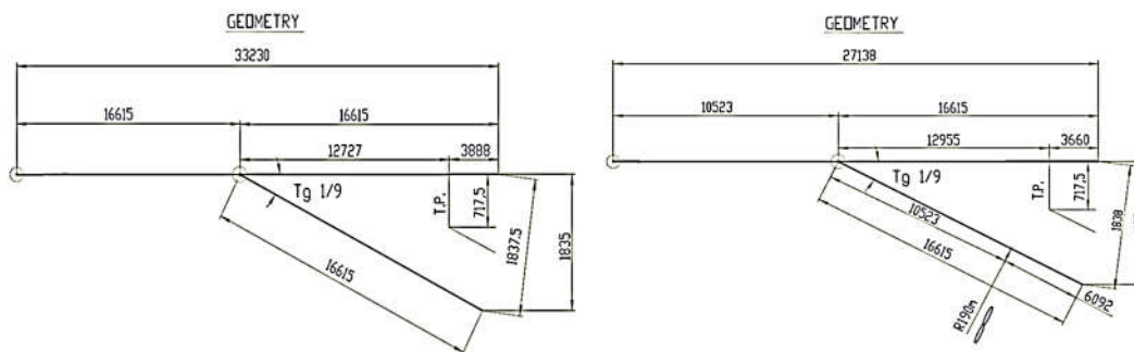
Figure 3. Geometrical specifications for turnouts with radii of 300m (left) and 190m (right)
