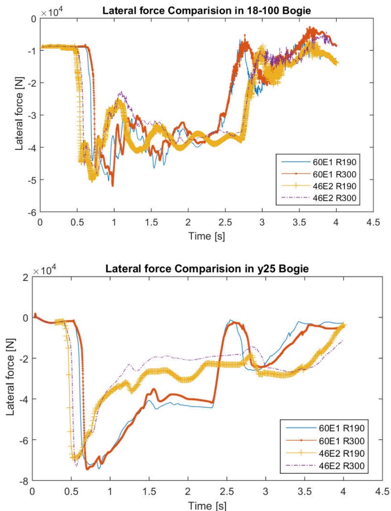
Figure 6. The calculated lateral forces for the two types of bogies on different turnouts
