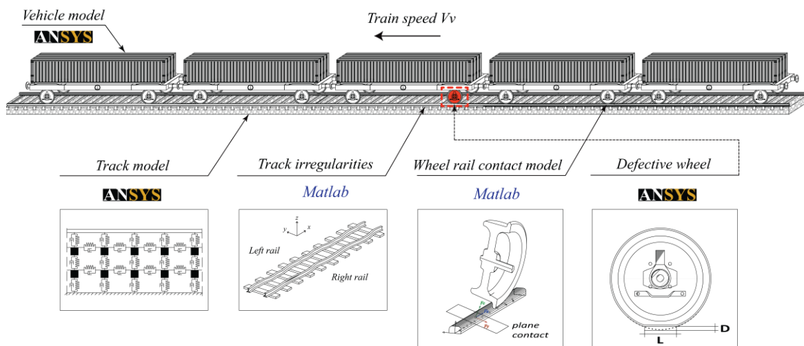
Figure 3. Train-track system
